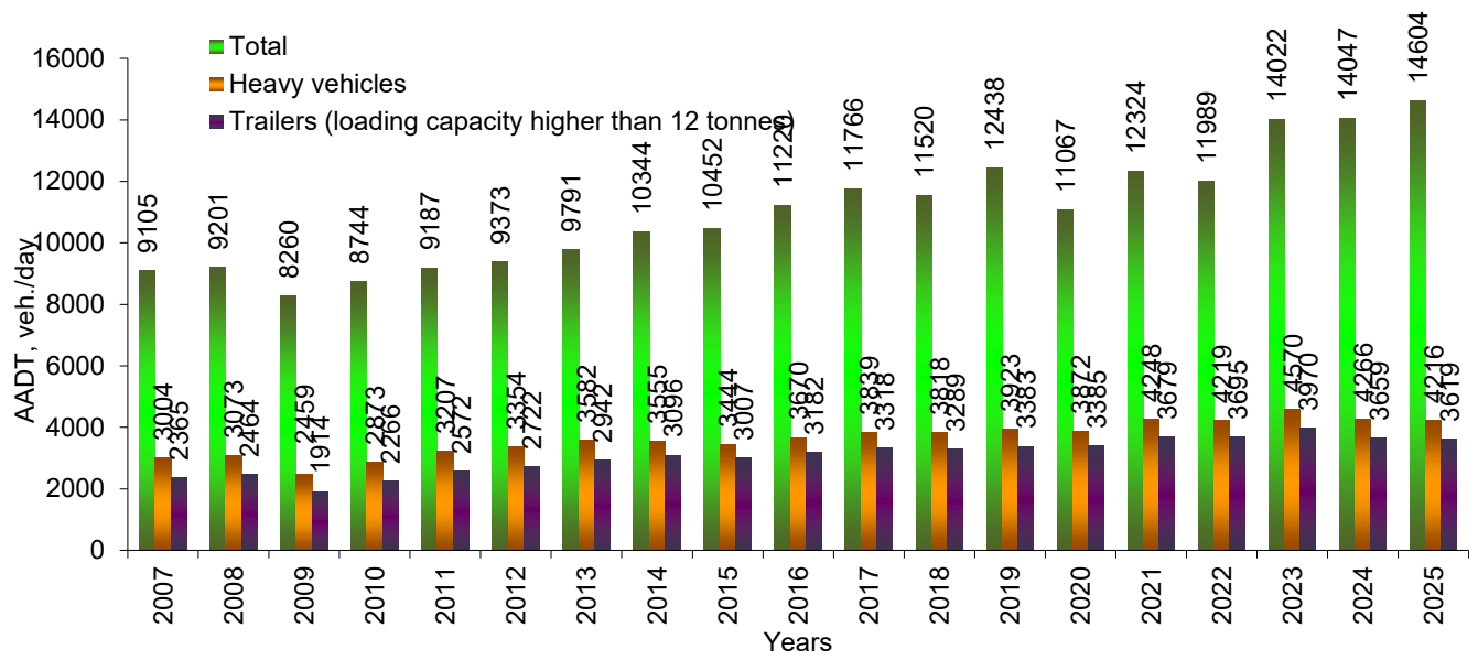
Change of annual average daily traffic (AADT) on the transport corridor Via Baltica since 2007
