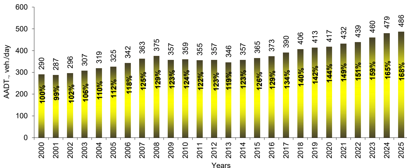
Change of annual average daily traffic (AADT) on the regional roads, compared to the year 2000
