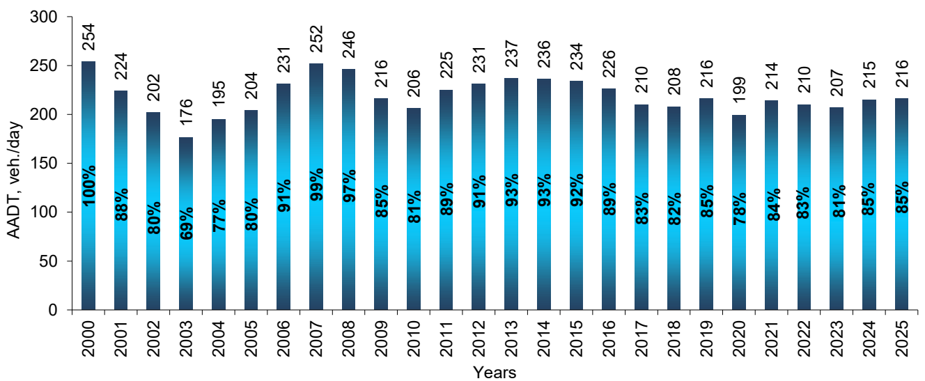
Change of heavy vehicles' annual average daily traffic (AADT) on the national roads, compared to the year 2000
