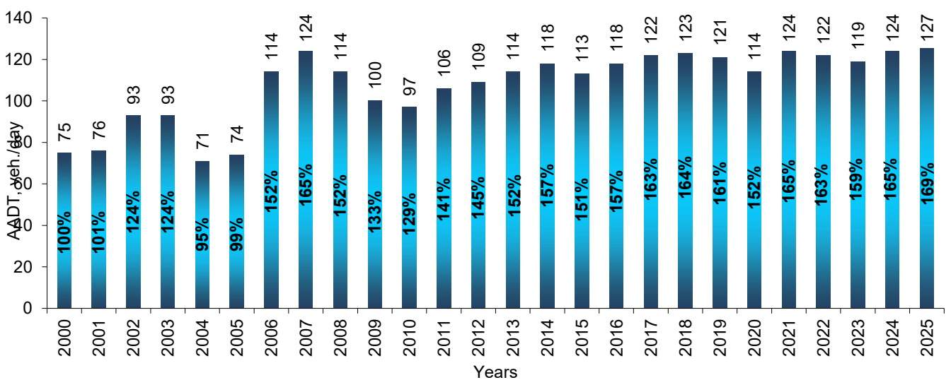
Change of trailer (loading capacity higher than 12 tonnes) average daily traffic (AADT) on the national roads, compared to the year 2000
