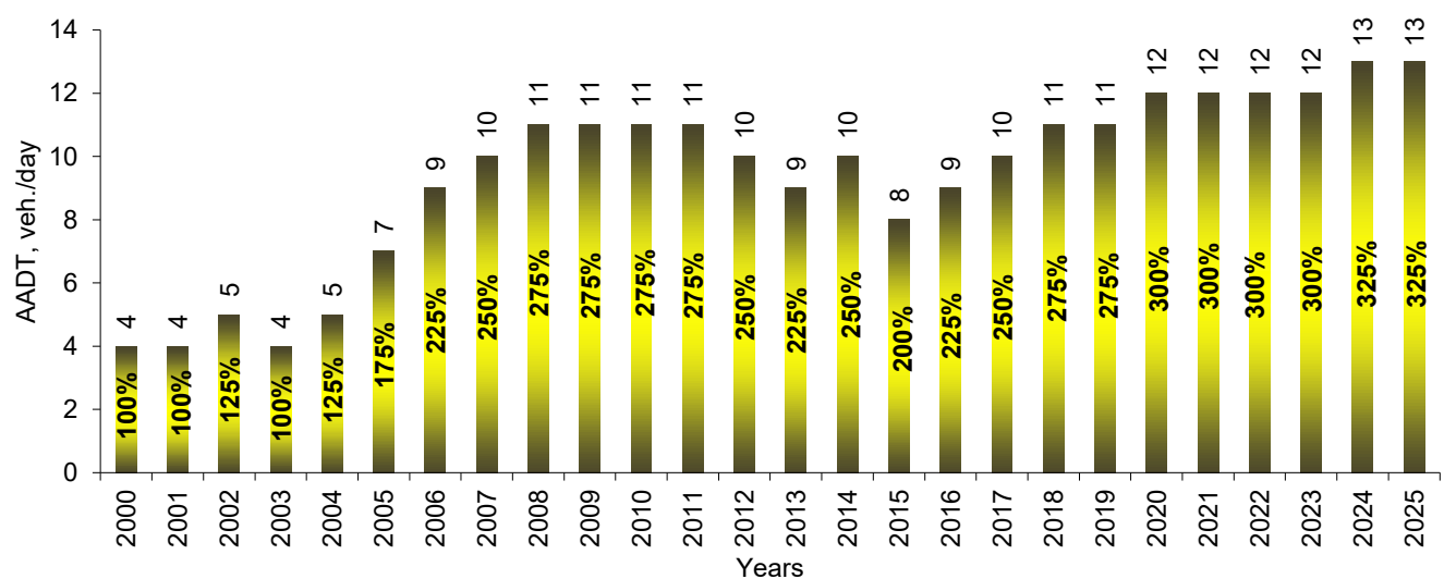
Change of trailer (loading capacity higher than 12 tonnes) annual average daily traffic (AADT) on the regional roads, compared to the year 2000
