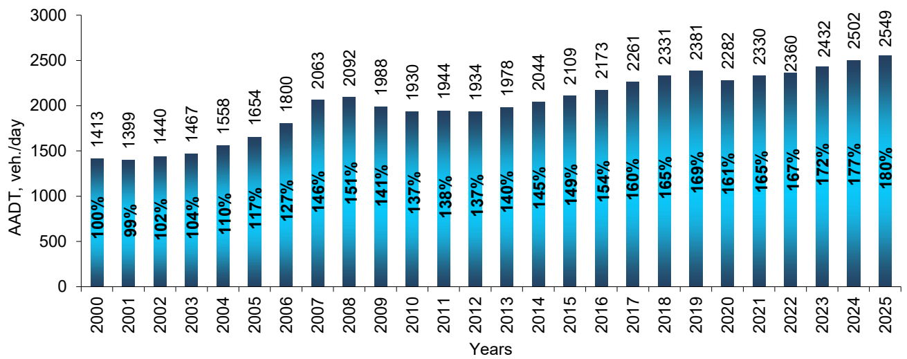
Change of annual average daily traffic (AADT) on the national roads, compared to the year 2000
